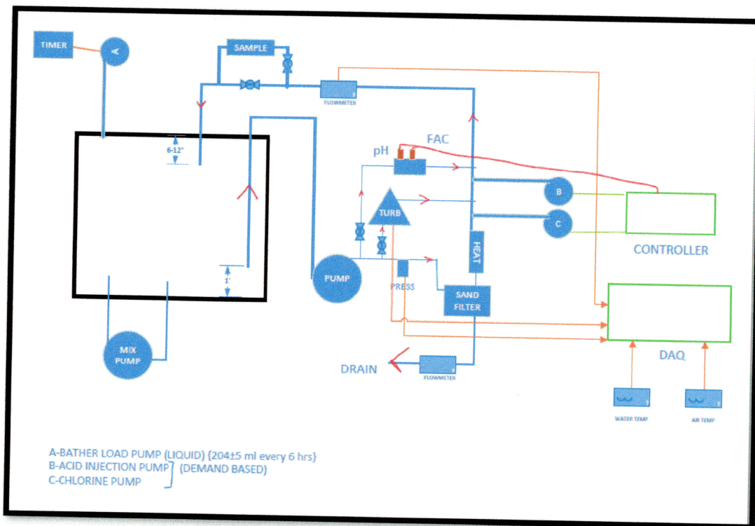
Figure 8- Test Setup
